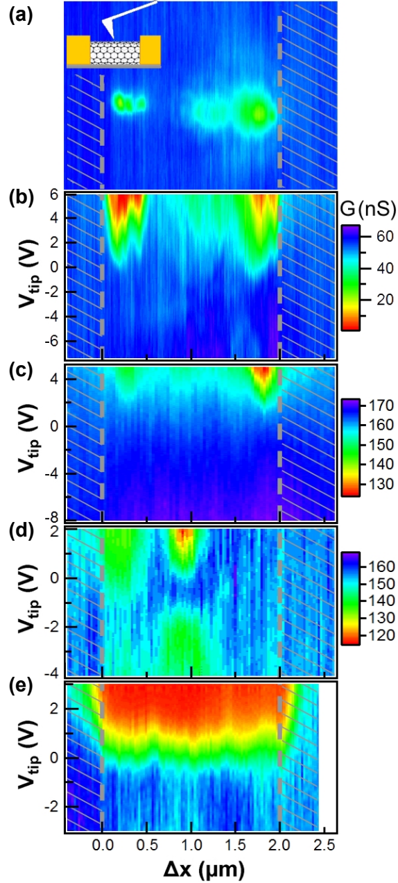
FIG. 1. (color online) (a) SGM and (b) corresponding SGS image of a s-SWNT having Schottky barriers at both electrodes and an additional, weakly-scattering defect in the channel at \Delta x = 1.2 \mu\text{m} . Approximate position of source and drain electrodes are indicated with grey striping. Inset depicts the measurement geometry. (c) SGS for a similar s-SWNT over a different range of V_{\text{tip}} . (d) SGS image for a strongly-scattering defect in a SWNT with only one sensitive interface. (e) SGS image for a pristine, small-bandgap SWNT that exhibits no appreciable Schottky barriers.
