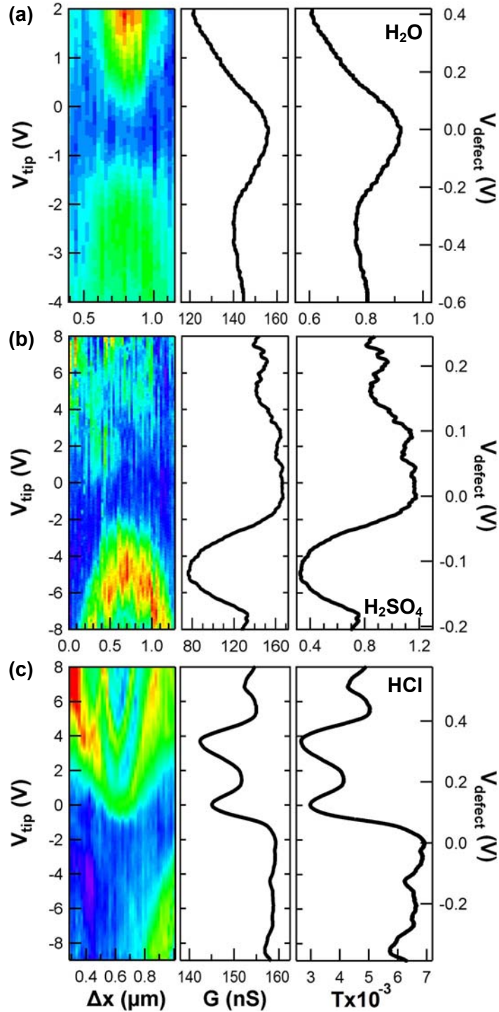
FIG. 3. (color online) Characteristic data for s-SWNTs point functionalized in (a) H 2 O, (b) H 2 SO 4 , and (c) HCl. Each depicts a portion of an SGS data set surrounding the defect site, the maximal G(V_{tip}) measured directly over the defect, and a transmission function T(E) calculated from G(V_{tip}) and the contact resistance, as described in the text.
